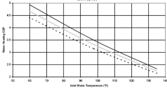
Water Heating COP vs. Inlet Water Temperature WH140 HT
