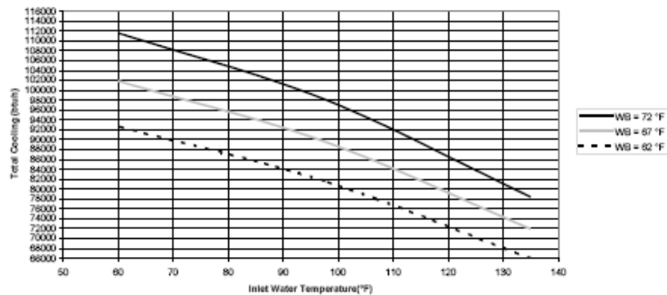
Cooling vs. Inlet Water Temperature WH140 HT
