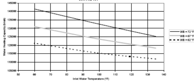
Water Heating Capacity vs. Inlet Water Temperature WH140 HT
